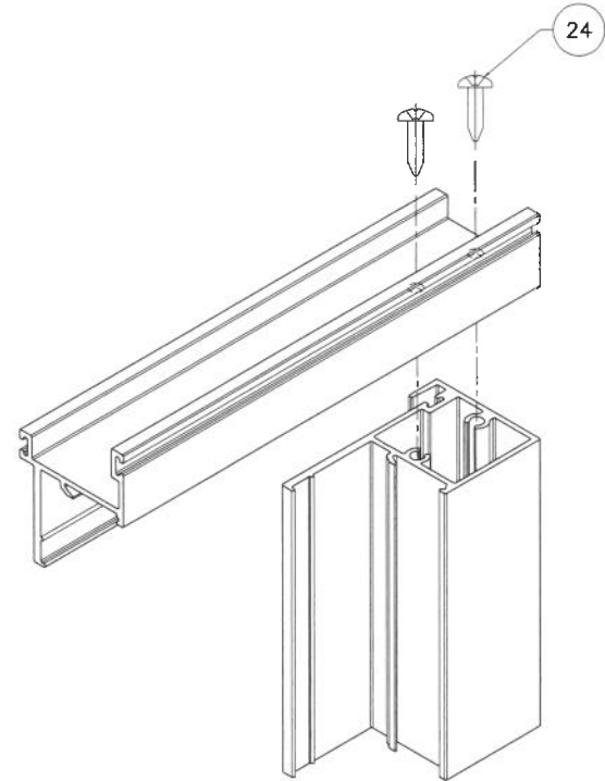
VENT TOP/BOTTOM ASSEMBLY
