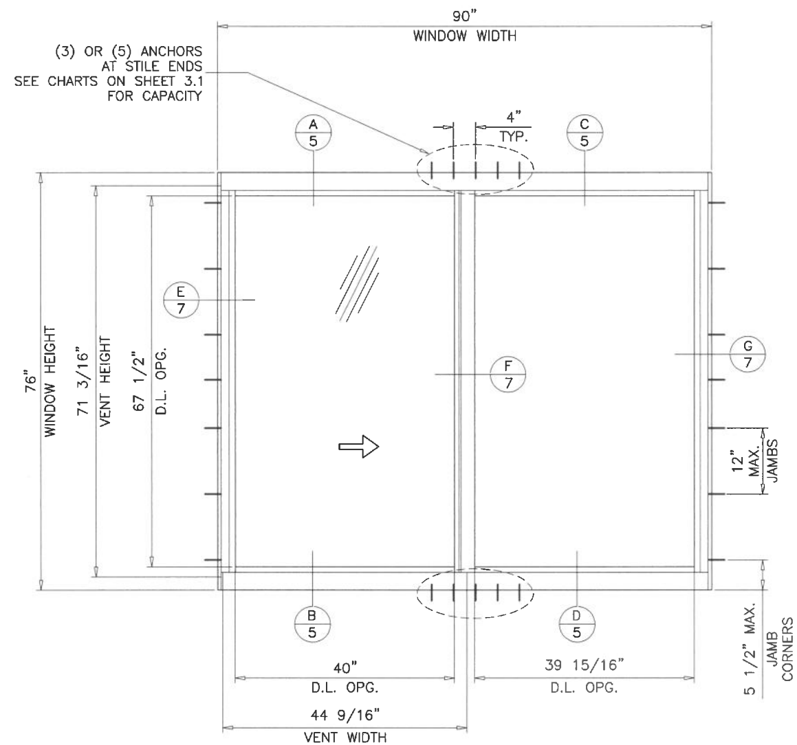
TYPICAL ELEVATION (TESTED UNIT)
