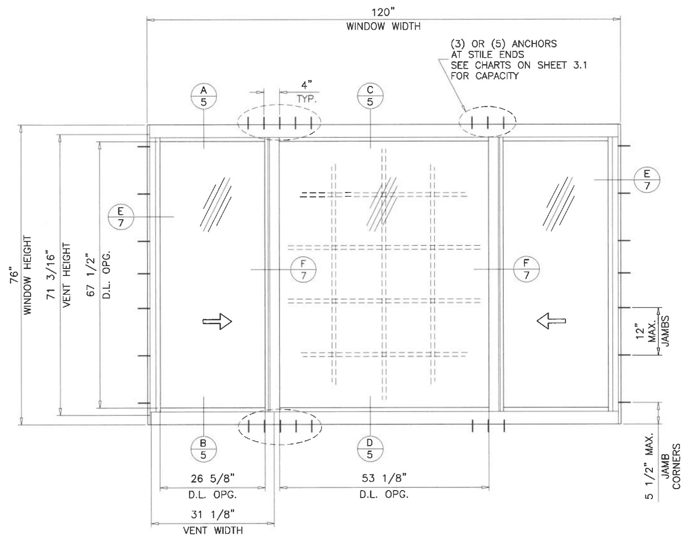
TYPICAL ELEVATION (TESTED UNIT)
